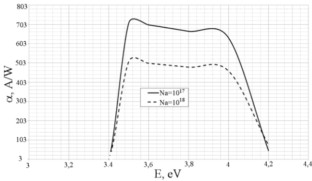
Fig. 12 – Phototransistor sensitivity vs quanta energy E , eV P = 10^{-3} \text{ W/cm}^2 and U = 9 \text{ V}
