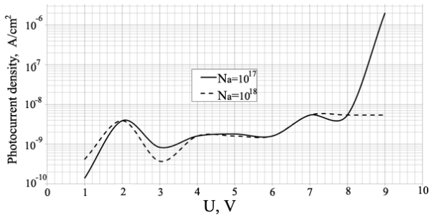
Fig. 6 – Dark current density j_{ph} vs the PT voltage
